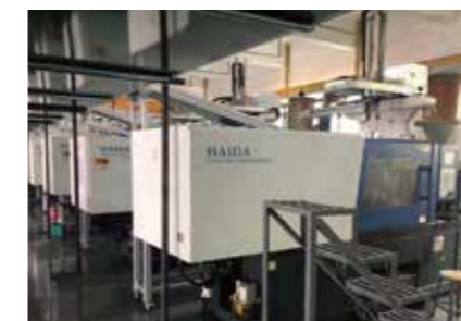
Injection Machine
